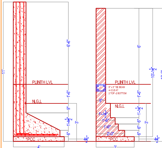
COLUMN SECTION
